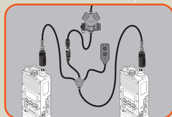
Dual radio config wired PTT interchangeable radio connection
